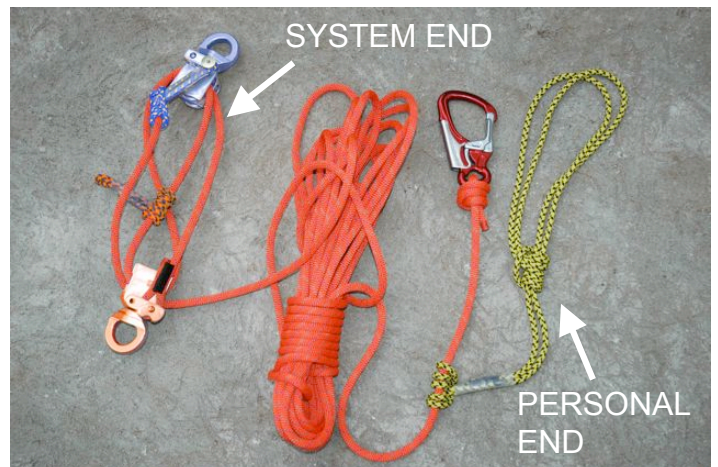
The Rock Exotica Omni AZTEK Elite® PERSONAL END shown on the right side with travel restrict/shock absorber and connecting auto locking carabiner. For instructions on this end see www.ropesthatrescue.com/aztek.htm
